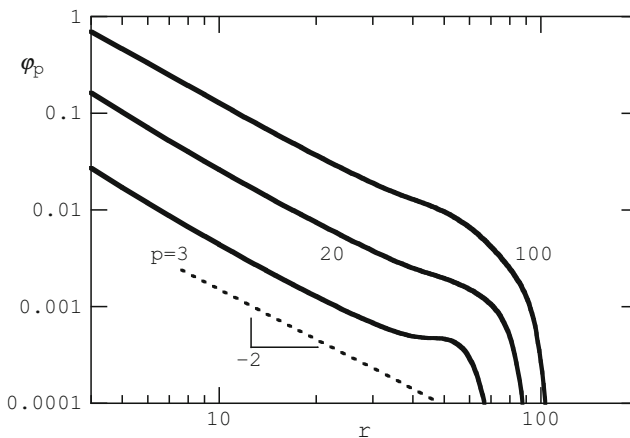
Fig. 9 Radial volume fraction profile \phi_p(r) (in log-log coordinates) for quenched PE stars with different numbers of branches p ; theta-solvent conditions; N = 200 , \alpha = 0.2 , D = 150 , \phi_s^b = 10^{-7} . The dotted line indicates the slope -2 , corresponding to a uniform extension of the branches
