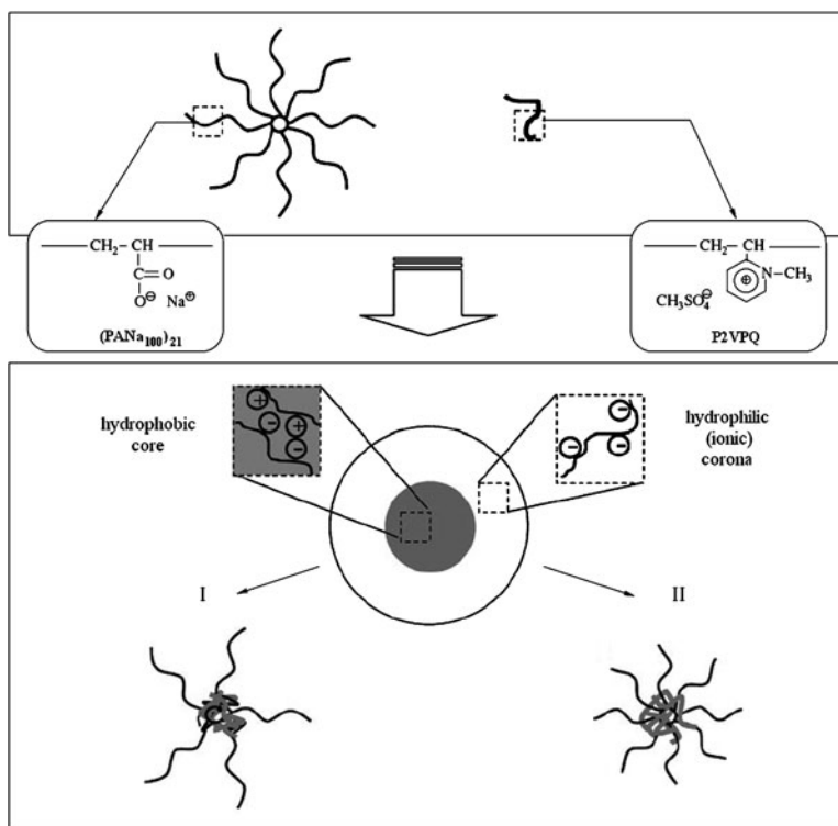
Fig. 4 Proposed inhomogeneous core–corona structure of the macromolecular co-assemblies formed in aqueous mixtures of (\text{PAA})_{21} stars (in the form of sodium salt) and \text{P2VPQ} . In structure I , some of the arms of the star-shaped HPE are embedded in the core and others are extended. In structure II , all of the arms contribute segments of equal length to the core. Reprinted from [80] with permission from Springer
