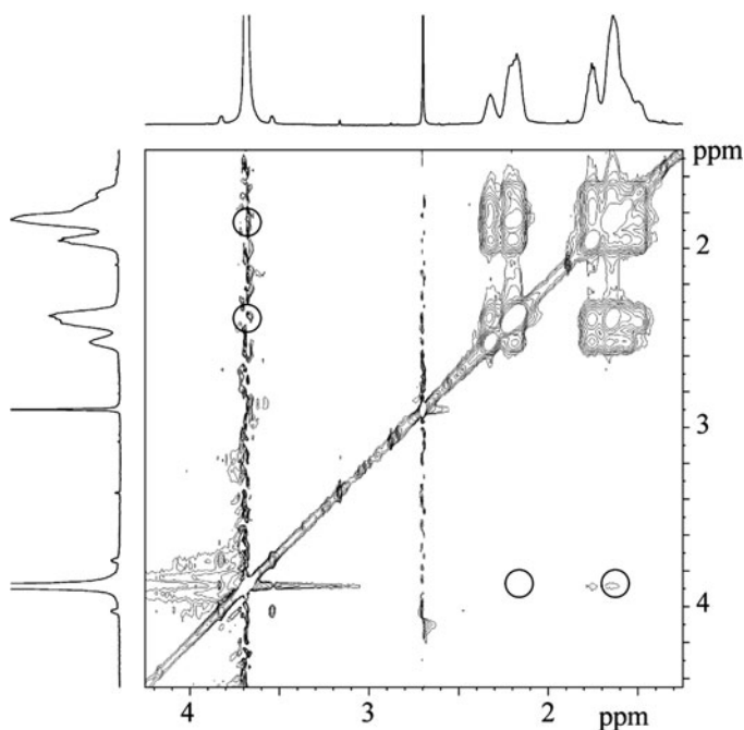
Fig. 6 2D 1 H NMR NOESY contour plot of a 1:1 mixture of PAA 42 - b -PAAm 417 and P2MVP 42 - b -PEO 446 in D 2 O at 1 mM NaNO 3 ( f_+ = 0.50 ). The circles indicate where cross-peaks would appear in case of close contact between PAAm and PEO chains. Adapted from [16]
